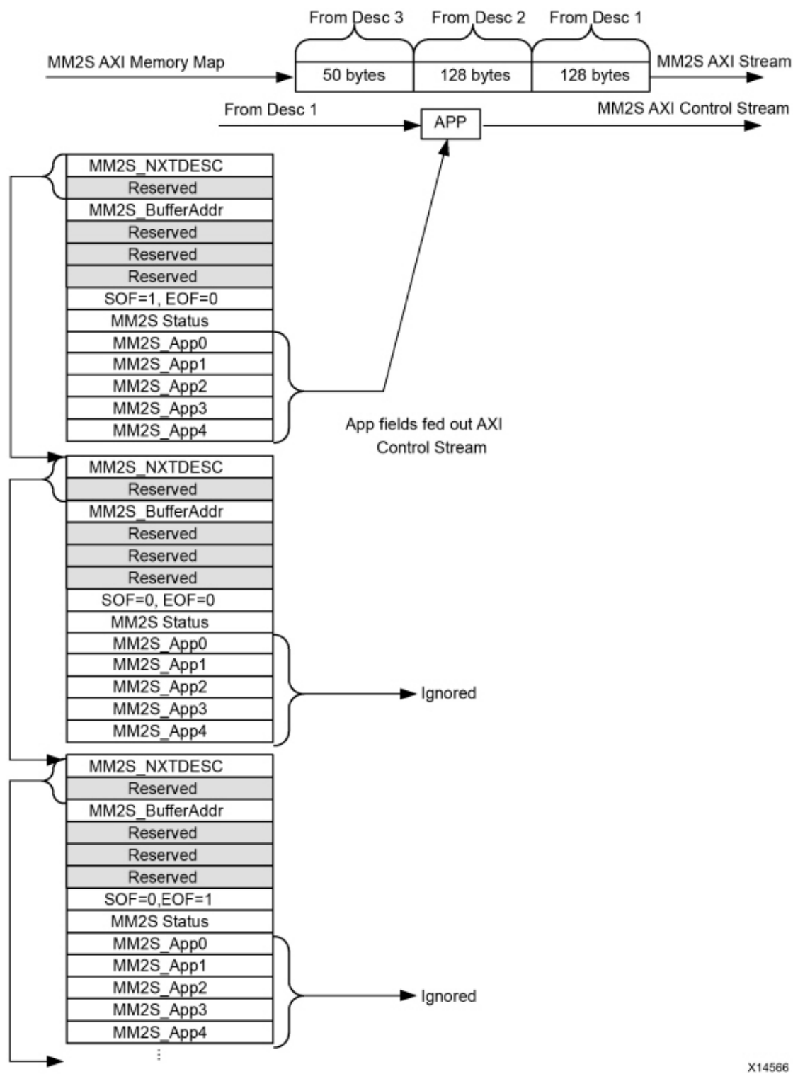
Figure: Detail of Descriptor Relationship to MM2S Stream and Control Stream
