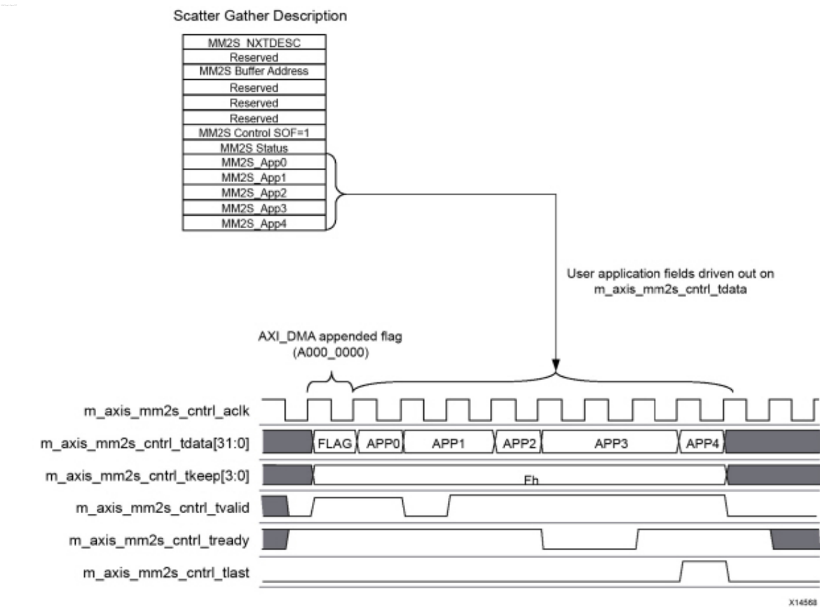
Figure: Example User Application Field / Timing for MM2S Control Stream
