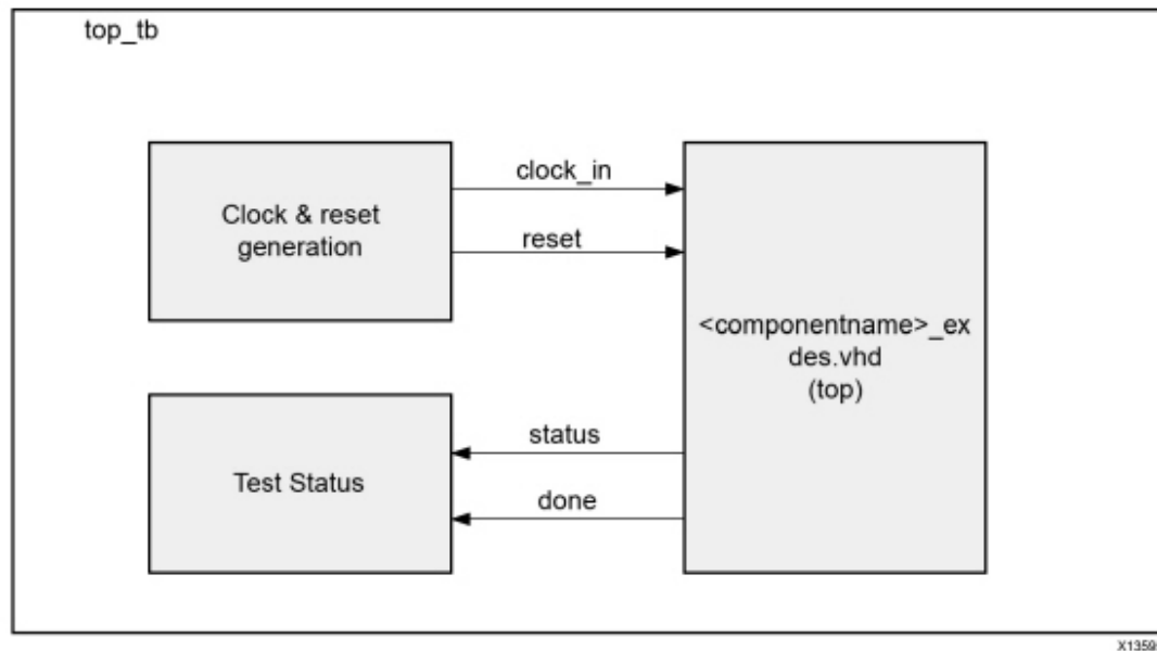
Figure: AXI DMA Example Design Test Bench
