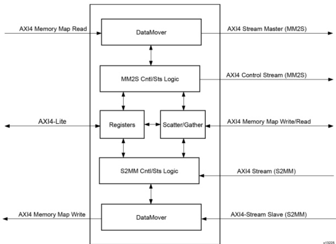
Figure: AXI DMA Block Diagram
