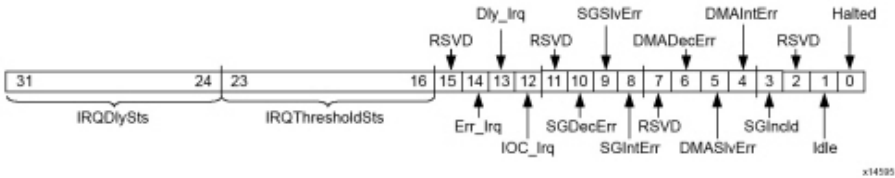
Figure: S2MM DMASR Register
