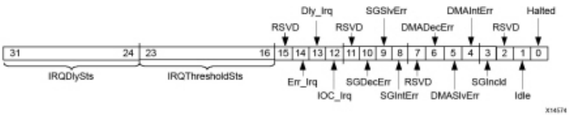
Figure: MM2S DMASR Register
