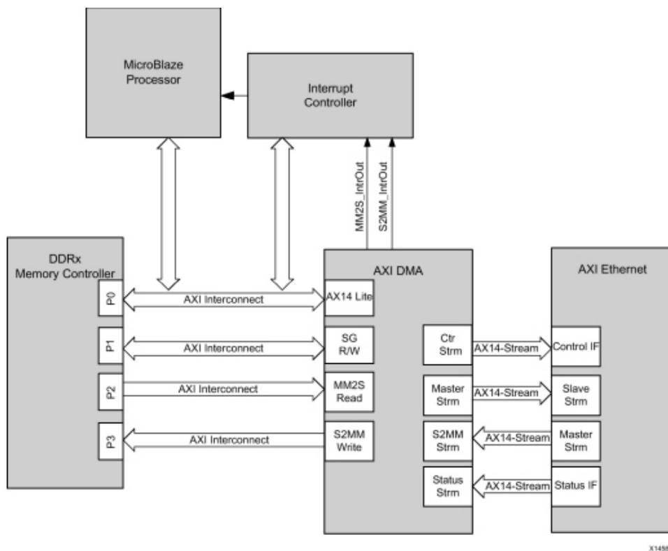
Figure: Typical MicroBlaze Processor System Configuration (AXI Ethernet)
