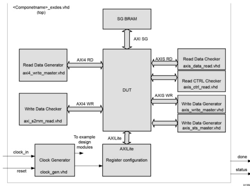
Figure: Block Diagram of Example Design
